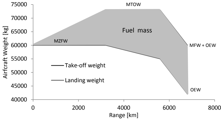
Figure 3.10: Take-off and Landing Weight Curve
