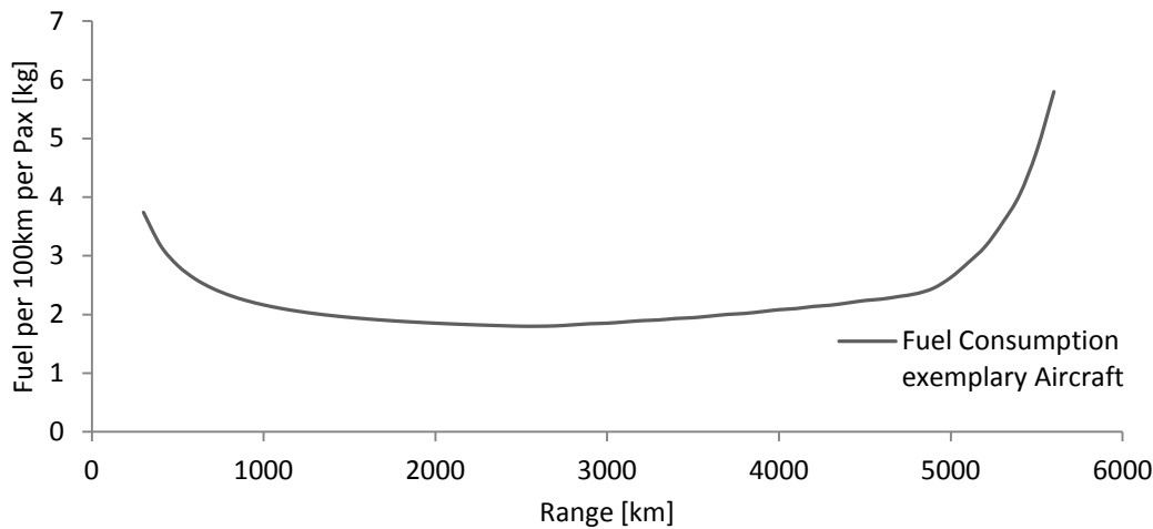
Figure 3.1: Bath Tub Curve of an exemplary Aircraft
