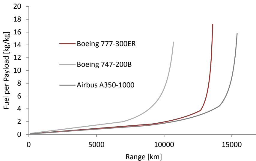
Figure 5.3: Comparison of Fuel per Kilogram Payload
